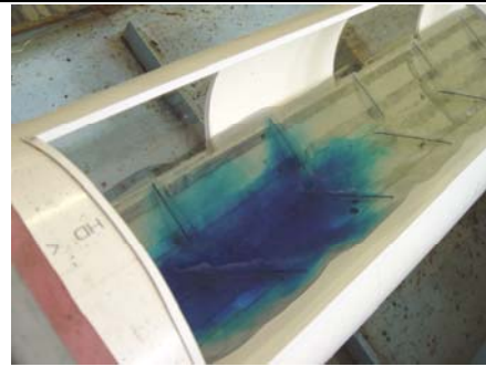
One standard baffle height flow depth: Dye inserted on right showing flow obstruction / shelter within baffle field on right (18/08/06)
