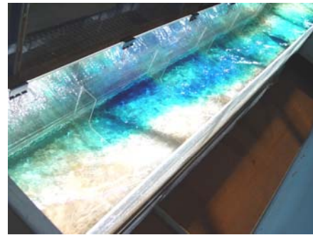
One standard baffle height flow depth: Time step 2; dye pattern showing flow retardance and fish shelter zone within baffle field on left (06/06/06)
