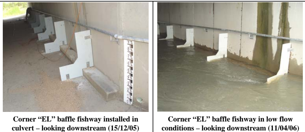
Box F5.1: Discovery Drive prototype corner “EL” baffle fishway on University Creek (Source: Ross Kapitzke)
