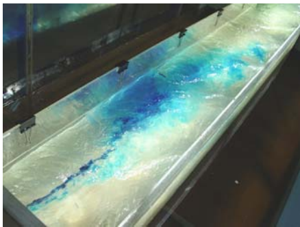
Three standard baffle height flow depth: Time step 1; dye pattern showing flow circulation within baffle field on left (06/06/06)
