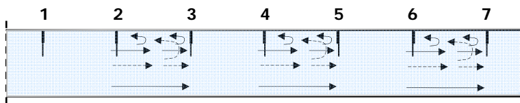
Two or more standard baffle height flow depth – submerged baffle leg flow condition
