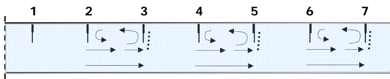
One standard baffle height flow depth – emerged baffle leg flow condition
