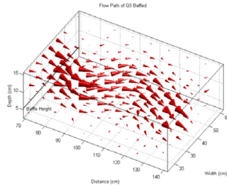
Graphical simulation of flow direction and magnitude obtained from fishway model
