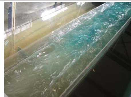
Three standard baffle height flow depth: Time step 2; showing spiralling flow on right hand oblong baffle side of fishway (06/06/06)
