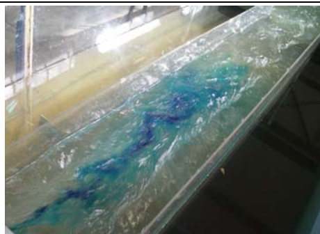
Three standard baffle height flow depth: Time step 1; dye pattern showing flow concentration in fishway centre (06/06/06)
