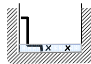
One standard baffle height flow depth – emerged baffle leg flow condition
