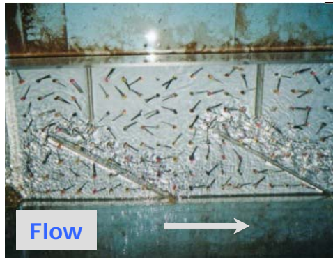
Flow direction vanes showing flow pattern in the lower flow layer within the baffle sets
