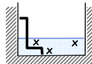
Two or more standard baffle height flow depth – submerged baffle leg flow condition
