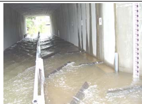
Offset baffle fishway and plain culvert barrel section – looking upstream (15/01/04)
