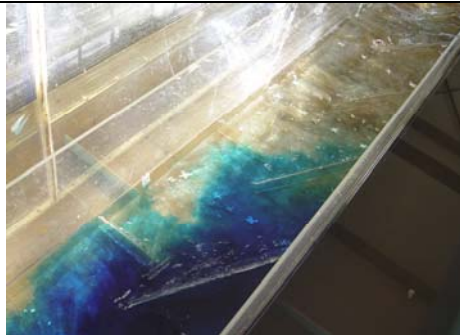
One standard baffle height flow depth: Time step 1; dye pattern showing flow circulation within baffle field (06/06/06)
