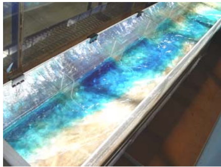
One standard baffle height flow depth: Time step 1; dye pattern showing flow retardance zone within baffle field on left and adjacent clear flow zone within barrel (06/06/06)
