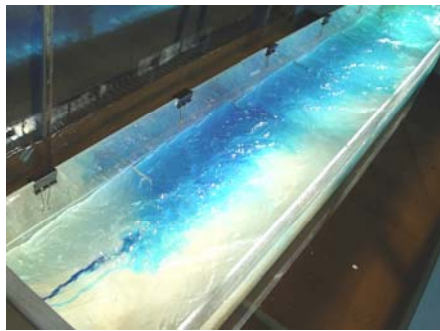
Three standard baffle height flow depth: Time step 2; showing flow retardance zone within baffle field on left and adjacent clear flow zone within barrel (06/06/06)
